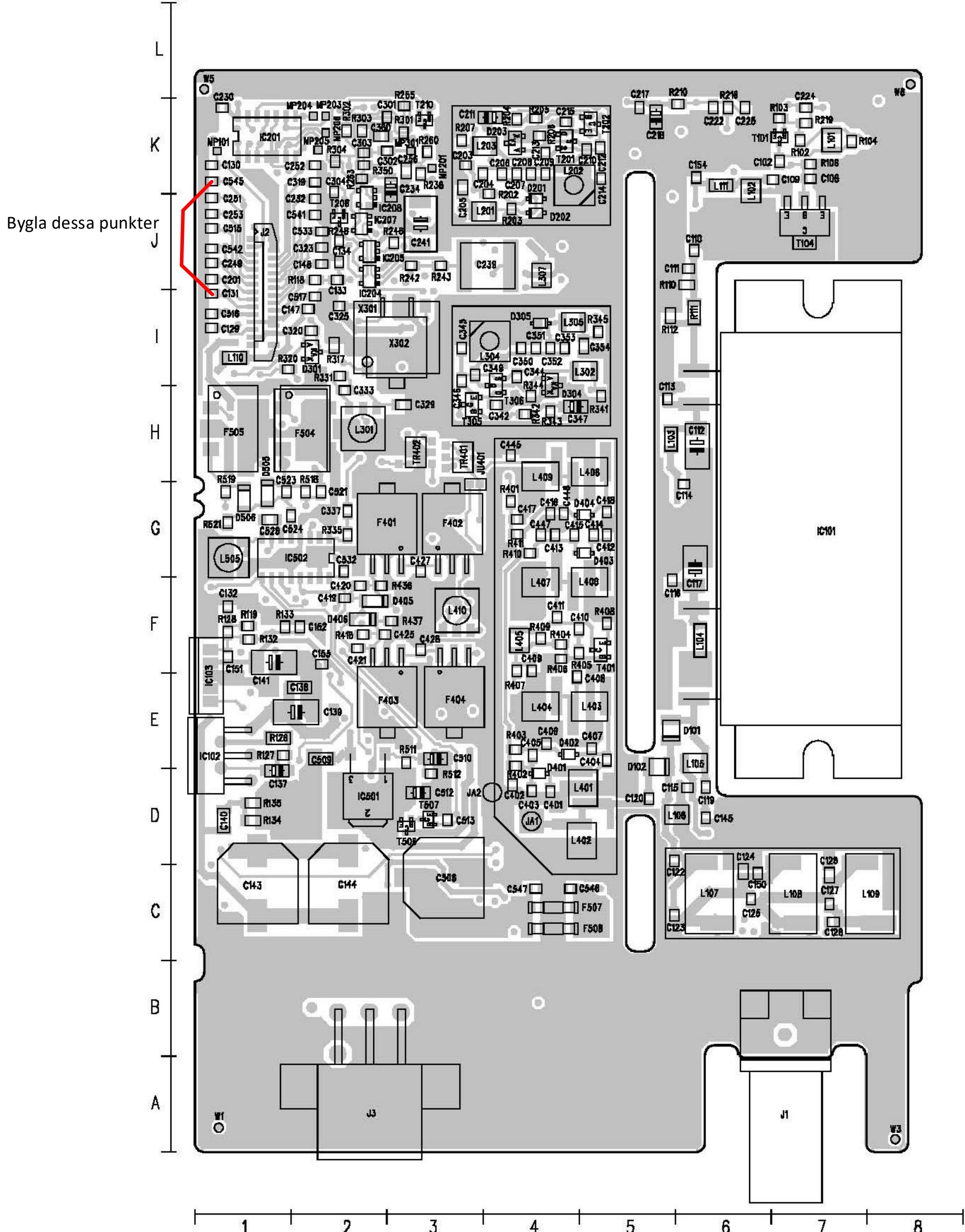
Componentside 776-5
